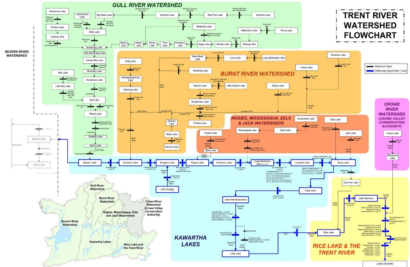
FIGURE A2 - Trent River Watershed Flow Chart
